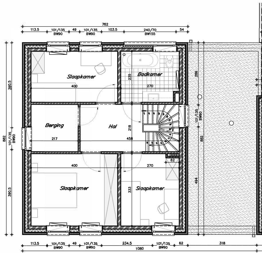
Verdiegingsplan
